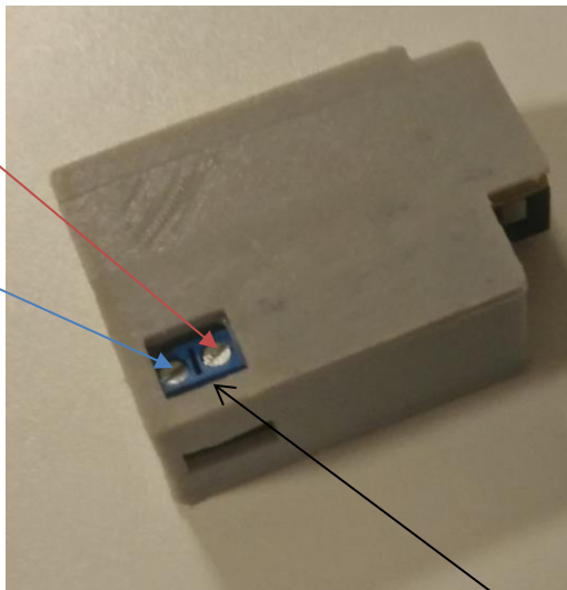
Optionale Stromversorgung (5V/500mA max) Optional power supply (5V/500mA max)
